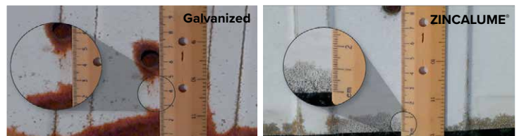
Corrosion comparison of a drip edge at 20 years of service life. Both products painted and located in an acid rain environment in Pennsylvania.
